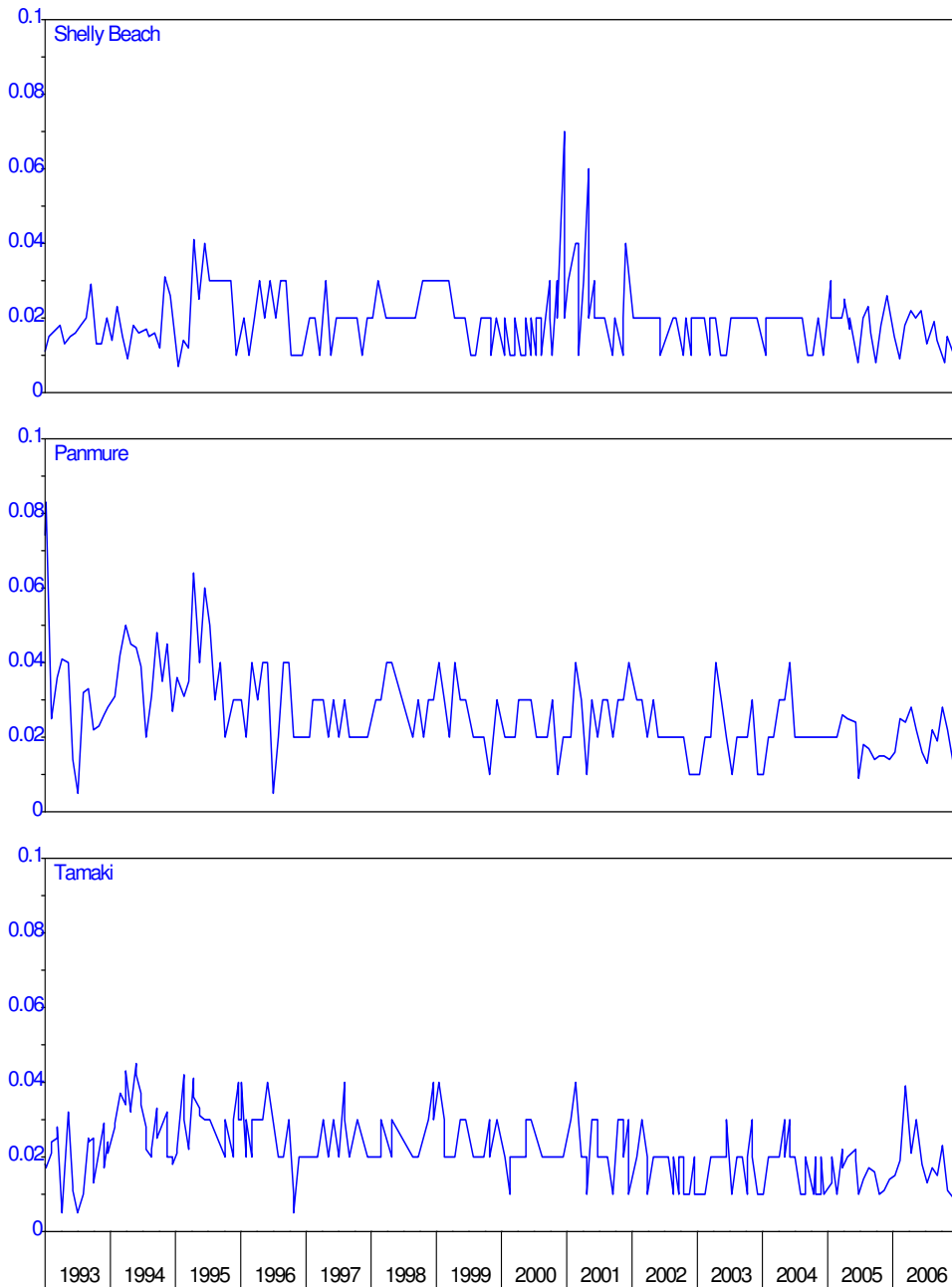
Figure 69: Kaipara harbour (Shelley beach) and Tamaki estuary – dissolved reactive phosphorus ( \text{gP}\cdot\text{m}^{-3} )
