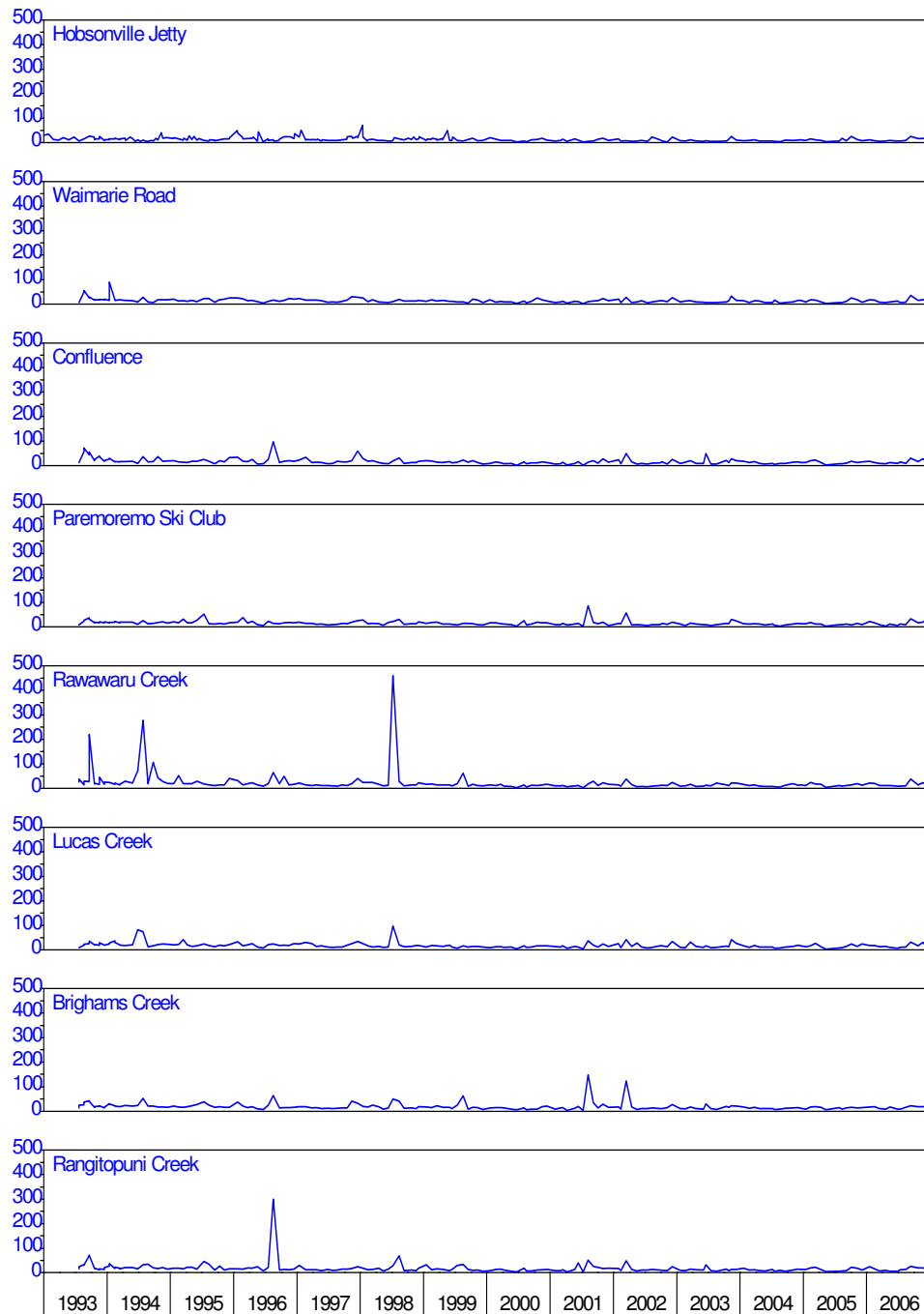
Figure 22: Upper Waitemata harbour – suspended solids (ppm)
