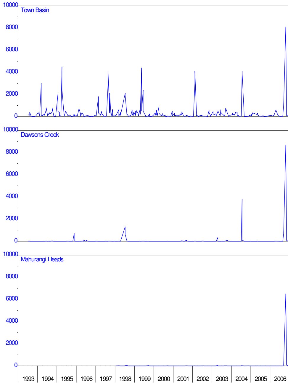
Figure 15: Mahurangi harbour – enterococci (cfu/100ml)
