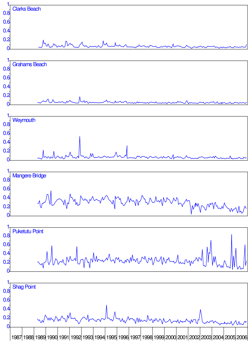
Figure 54: Manukau harbour – total phosphorus (g.m-3)
