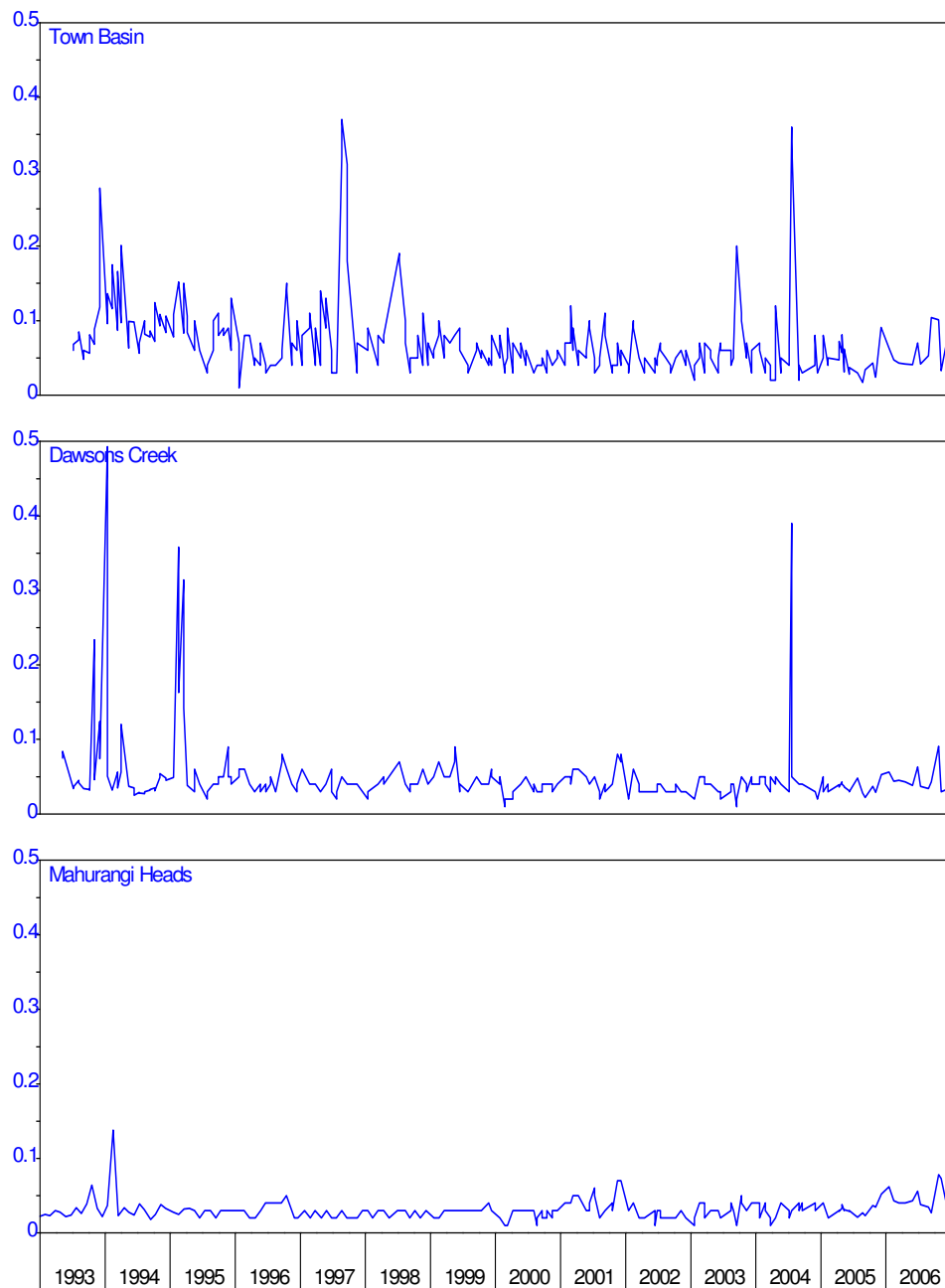
Figure 13: Mahurangi harbour – Total phosphorus ( \text{g.m}^{-3} )
