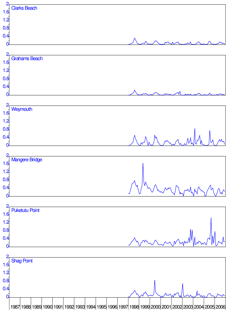
Figure 50: Manukau harbour – nitrate+nitrite (gN.m -3 )
