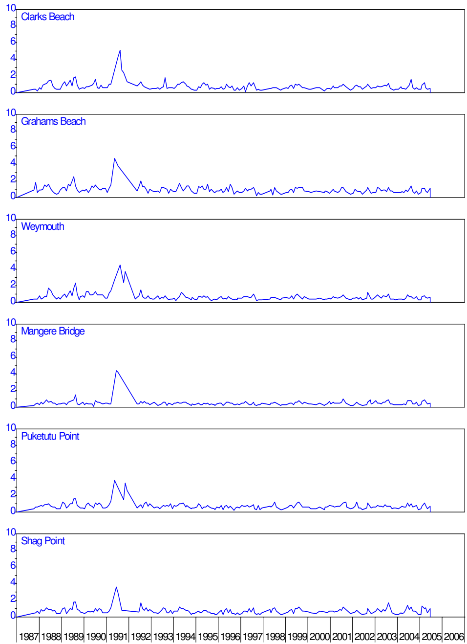
Figure 46: Manukau harbour – transparency (Secchi (m))
