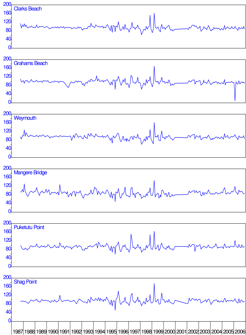
Figure 52: Manukau harbour – dissolved oxygen (% saturated)
