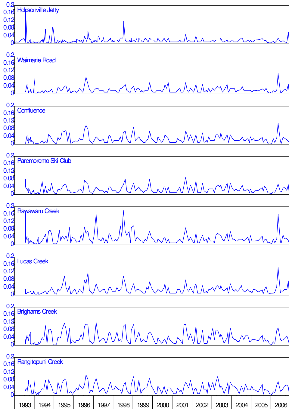
Figure 24: Upper Waitemata harbour – Ammoniacal nitrogen ( \text{gN.m}^{-3} )
