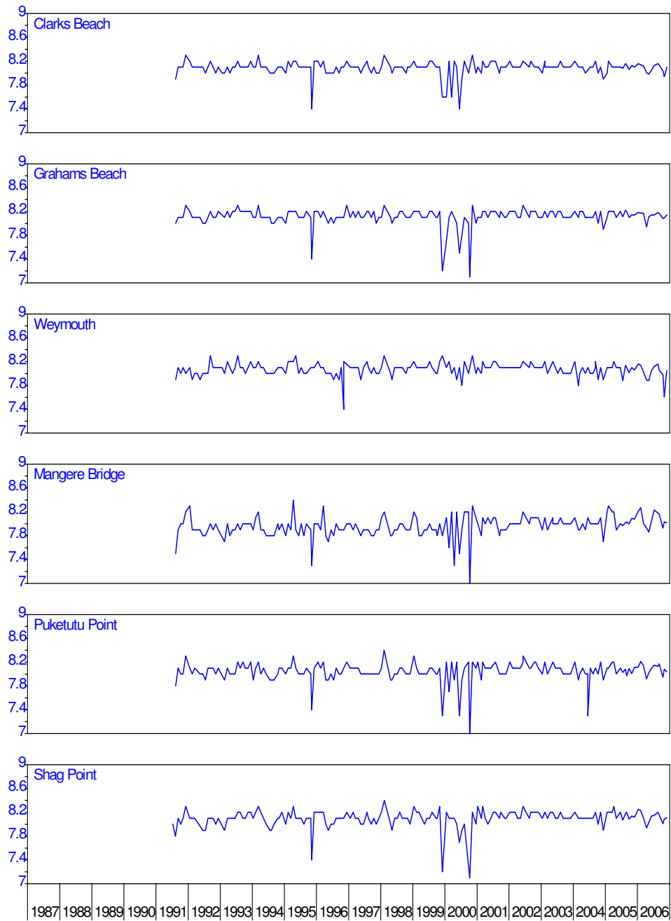
Figure 48: Manukau harbour - pH
