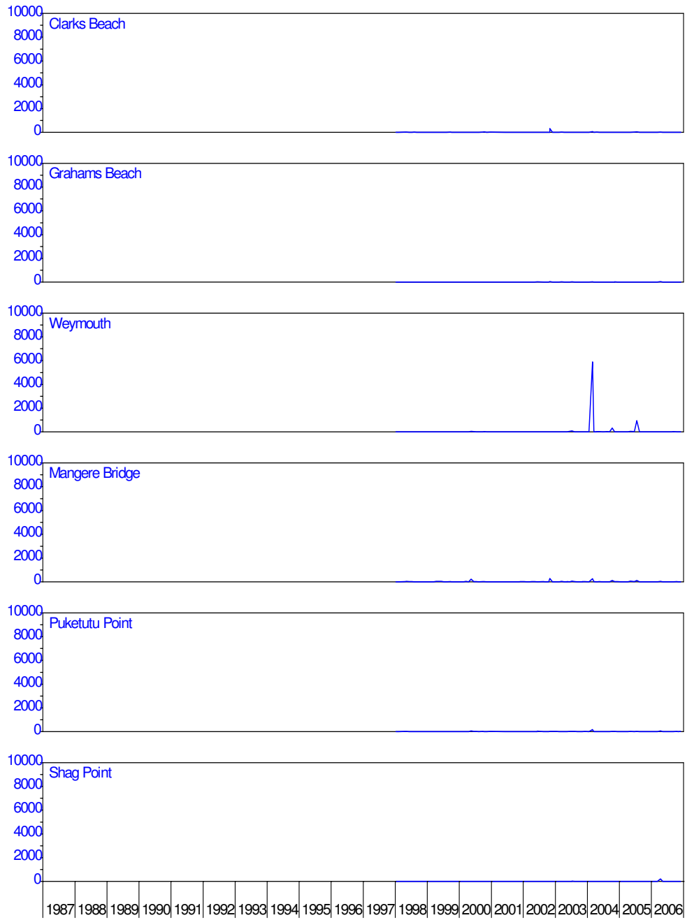
Figure 56: Manukau harbour – enterococci (cfu/100ml)
