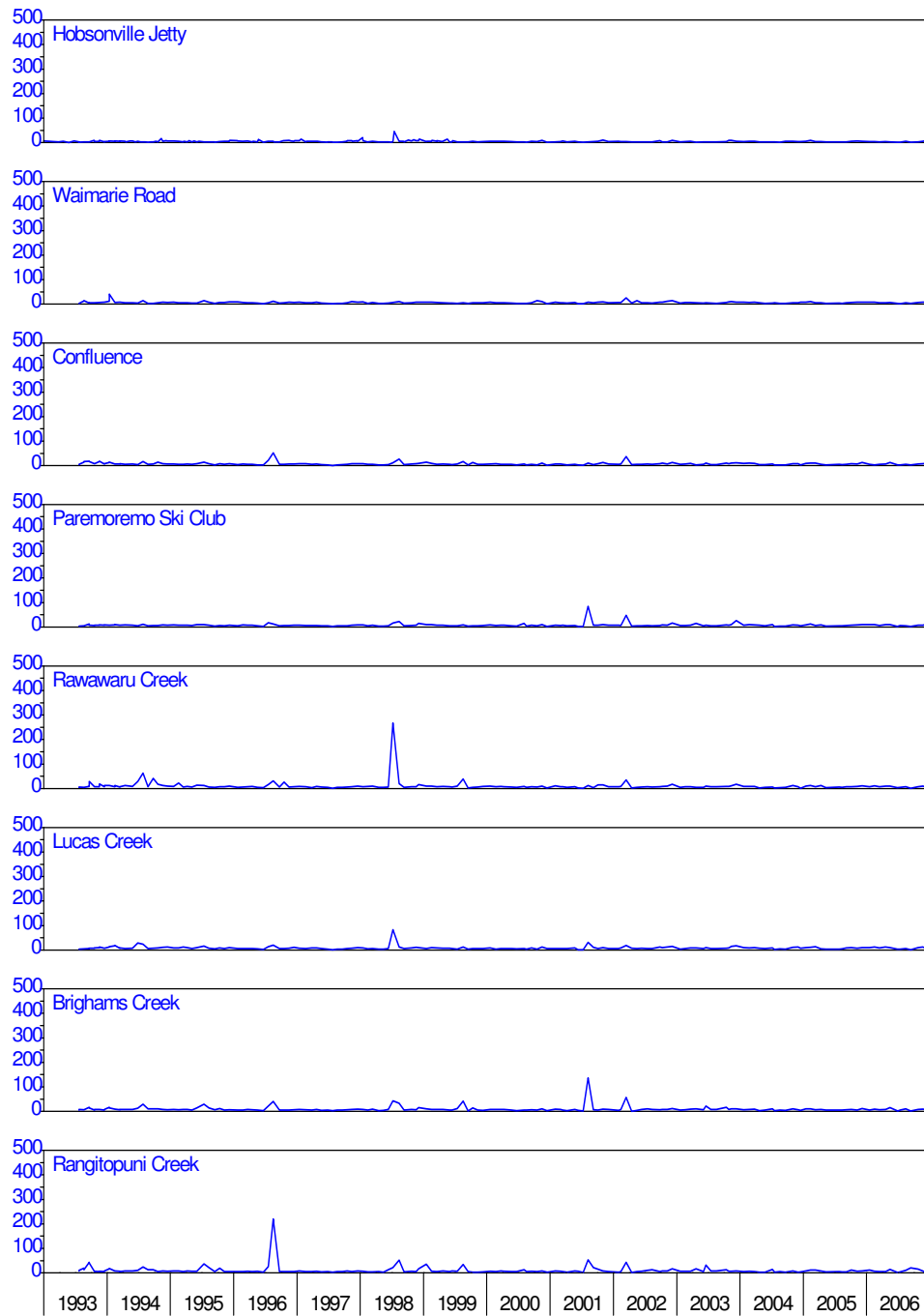
Figure 18: Upper Waitemata harbour – turbidity (NTU)
