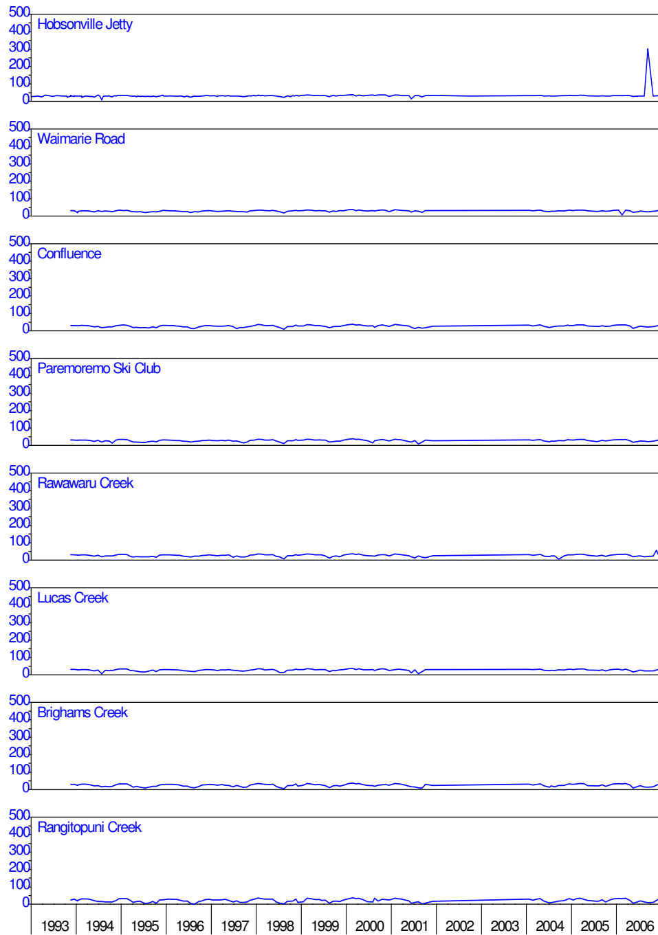
Figure 17 Upper Waitemata harbour – Salinity (ppt)
