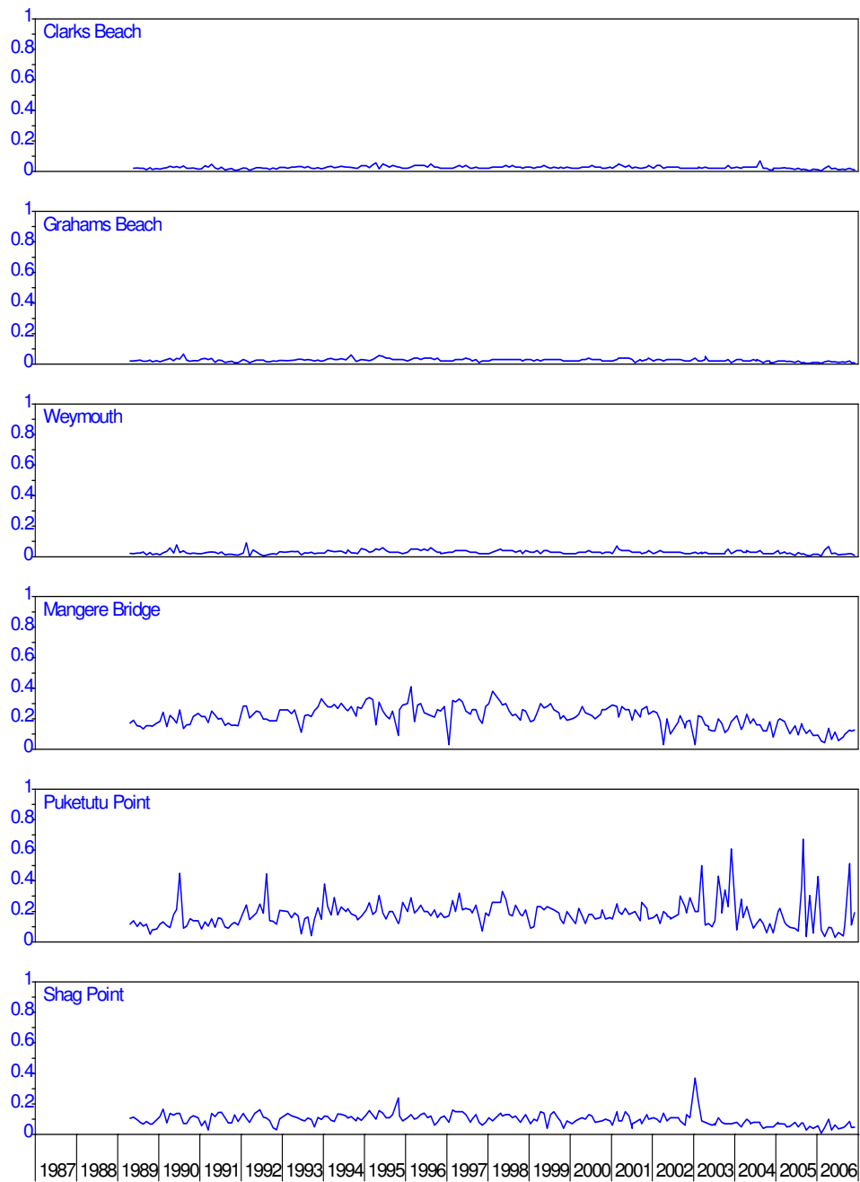
Figure 55: Manukau harbour – dissolved reactive phosphorus (gPm -3 )
