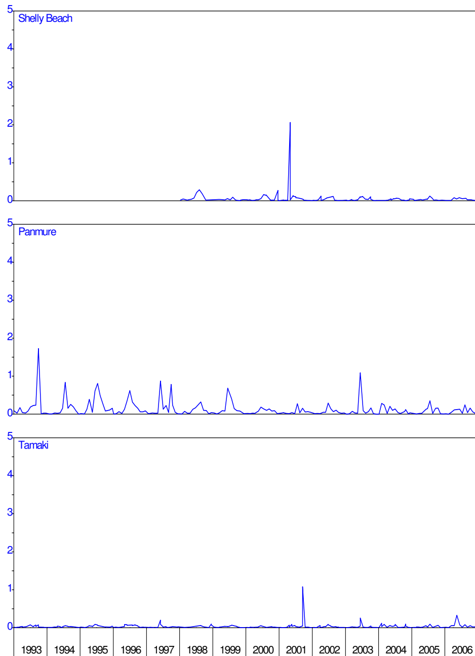
Figure 64: Kaipara harbour (Shelley beach) and Tamaki estuary – nitrate+nitrite ( \text{gN.m}^{-3} )
