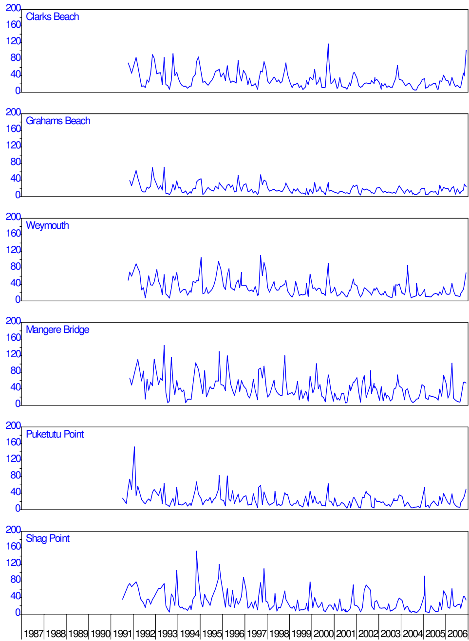
Figure 48: Manukau harbour – suspended solids (ppm)
