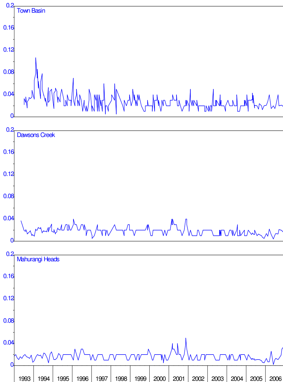
Figure 14: Mahurangi harbour – dissolved reactive phosphorus ( \text{gPm}^{-3} )
