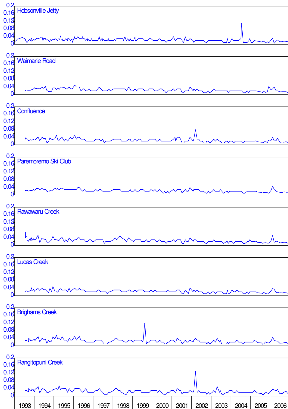
Figure 28: Upper Waitemata harbour – dissolved reactive phosphorus ( \text{gP}\cdot\text{m}^{-3} )
