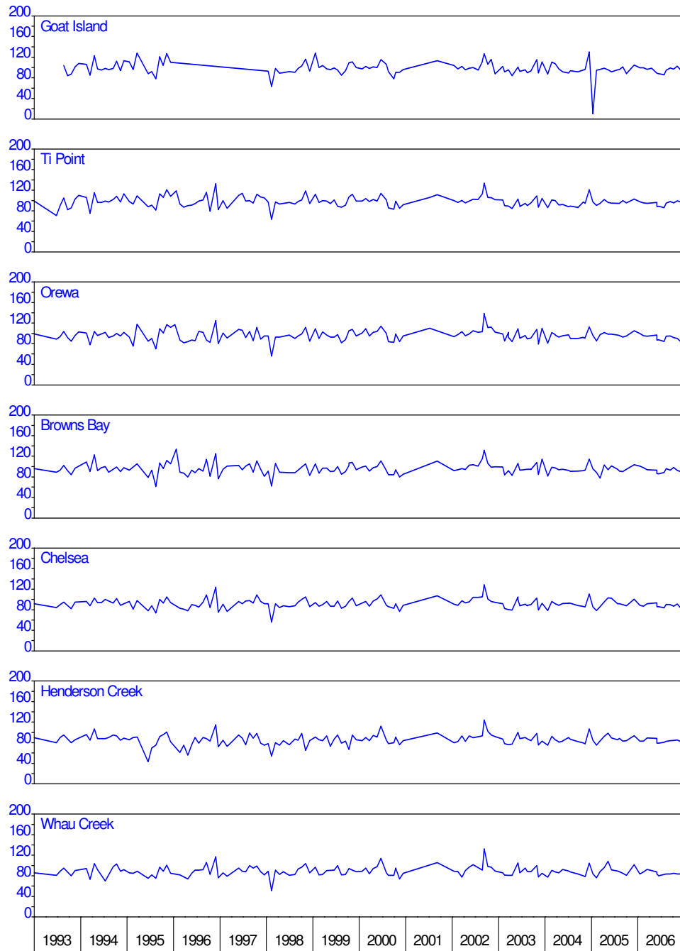
Figure 39: East Coast – dissolved oxygen (% saturated)
