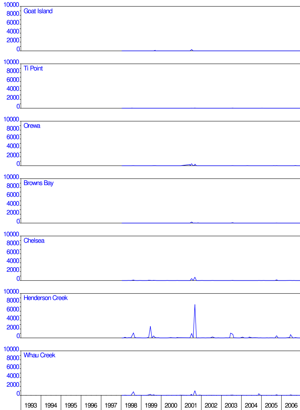
Figure 43: East Coast – enterococci (cfu/100ml)
