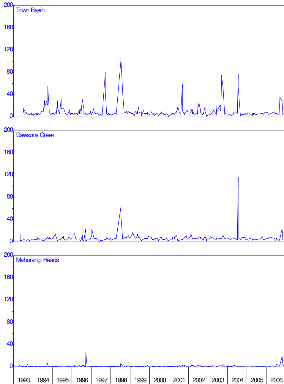
Figure 4: Mahurangi harbour – turbidity (NTU)
