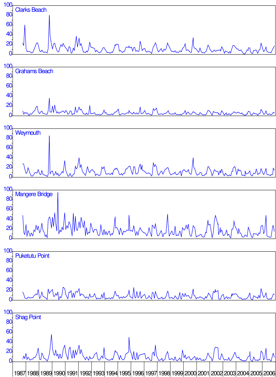
Figure 45: Manukau harbour – turbidity (NTU)
