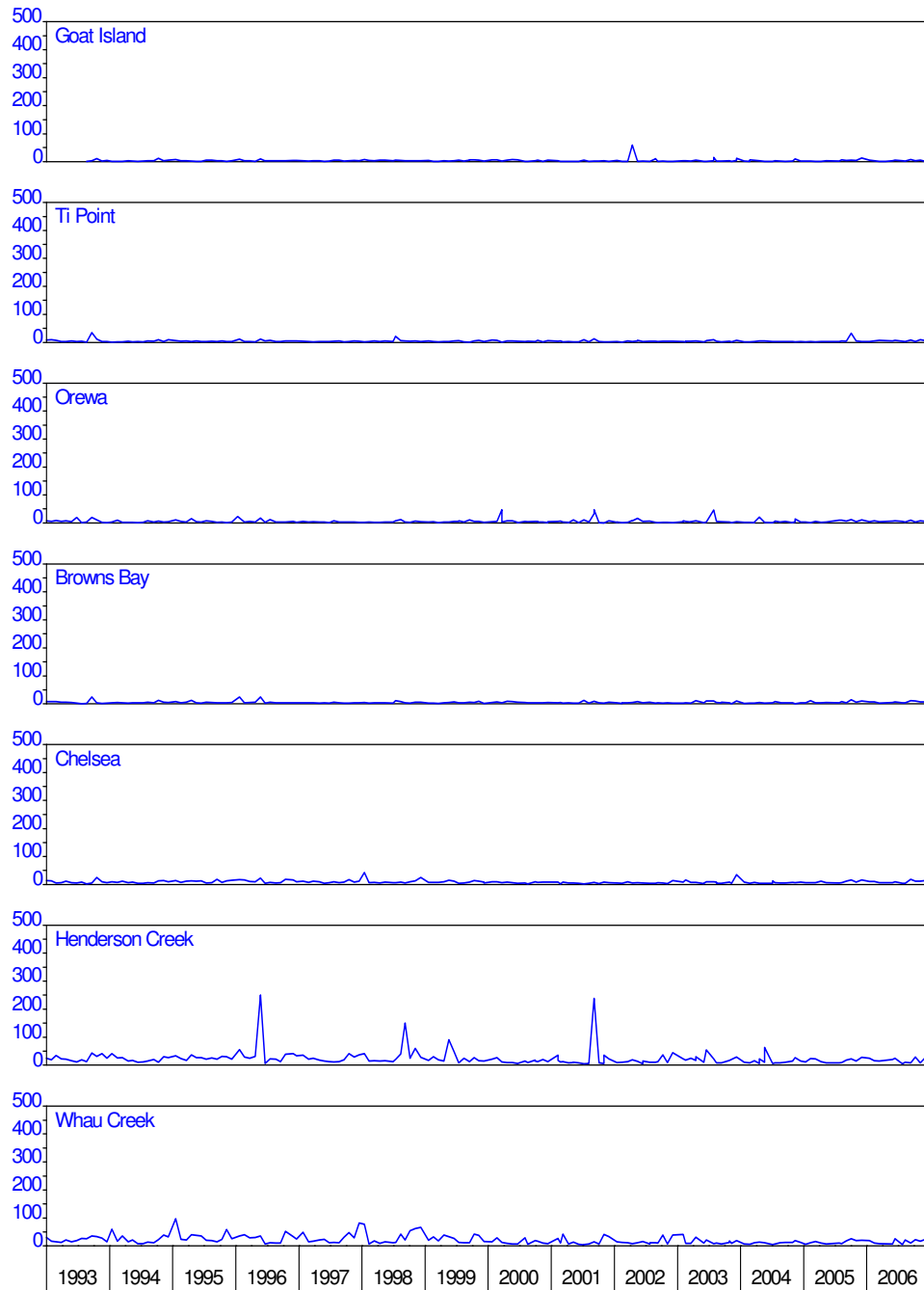
Figure 36: East Coast – suspended solids (ppm)
