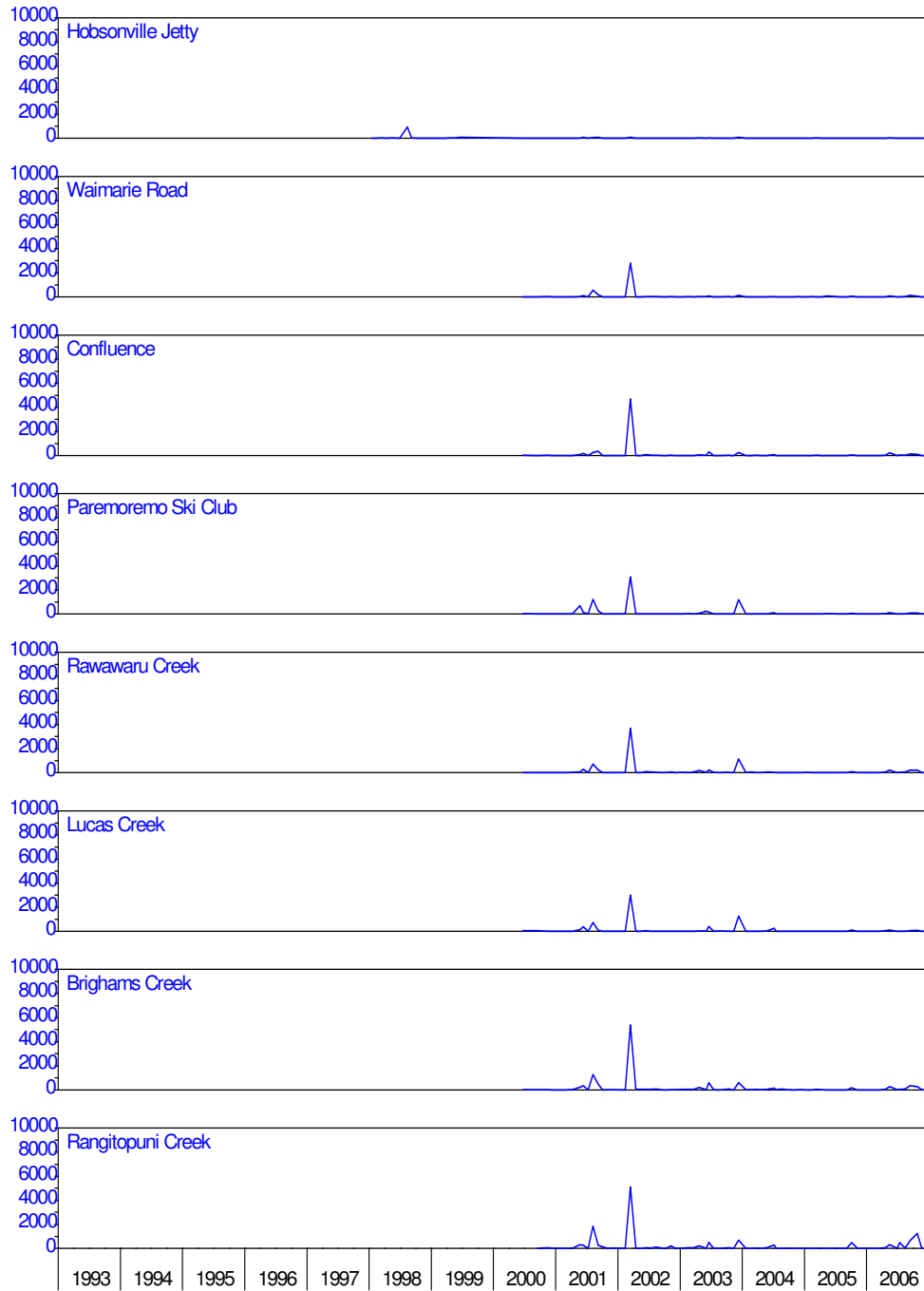
Figure 29: Upper Waitemata harbour – enterococci (cfu/100m)
