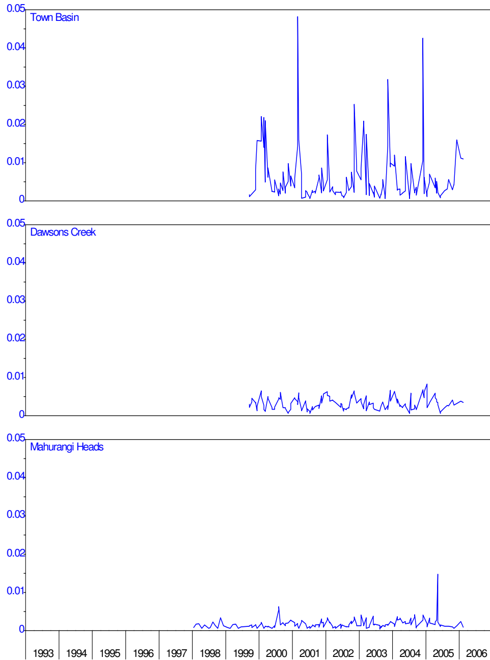
Figure 16: Mahurangi harbour – Chlorophyll a (ppm)
