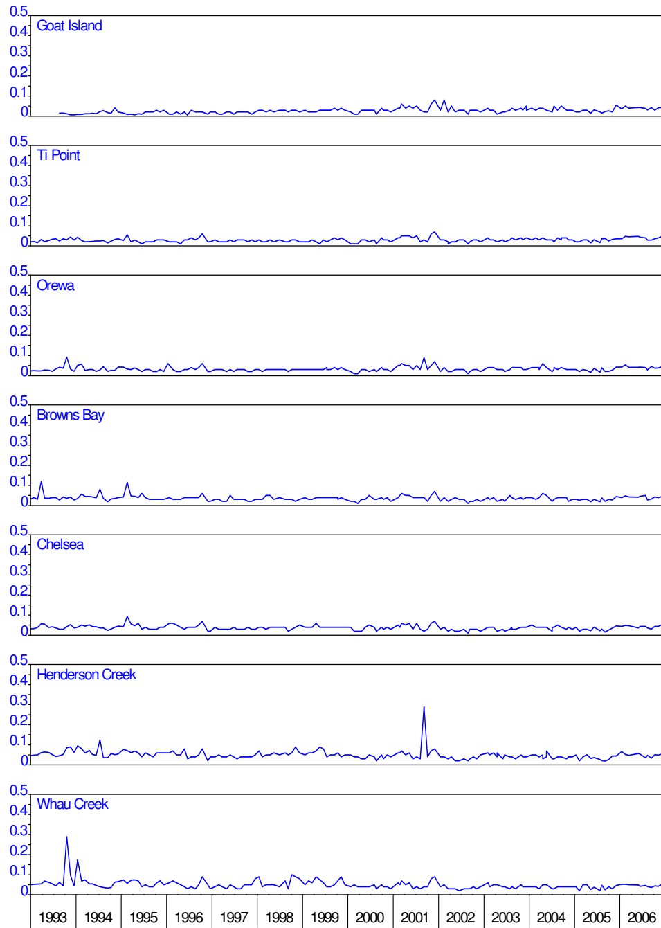
Figure 41: East Coast – total phosphorus (g.m-3)
