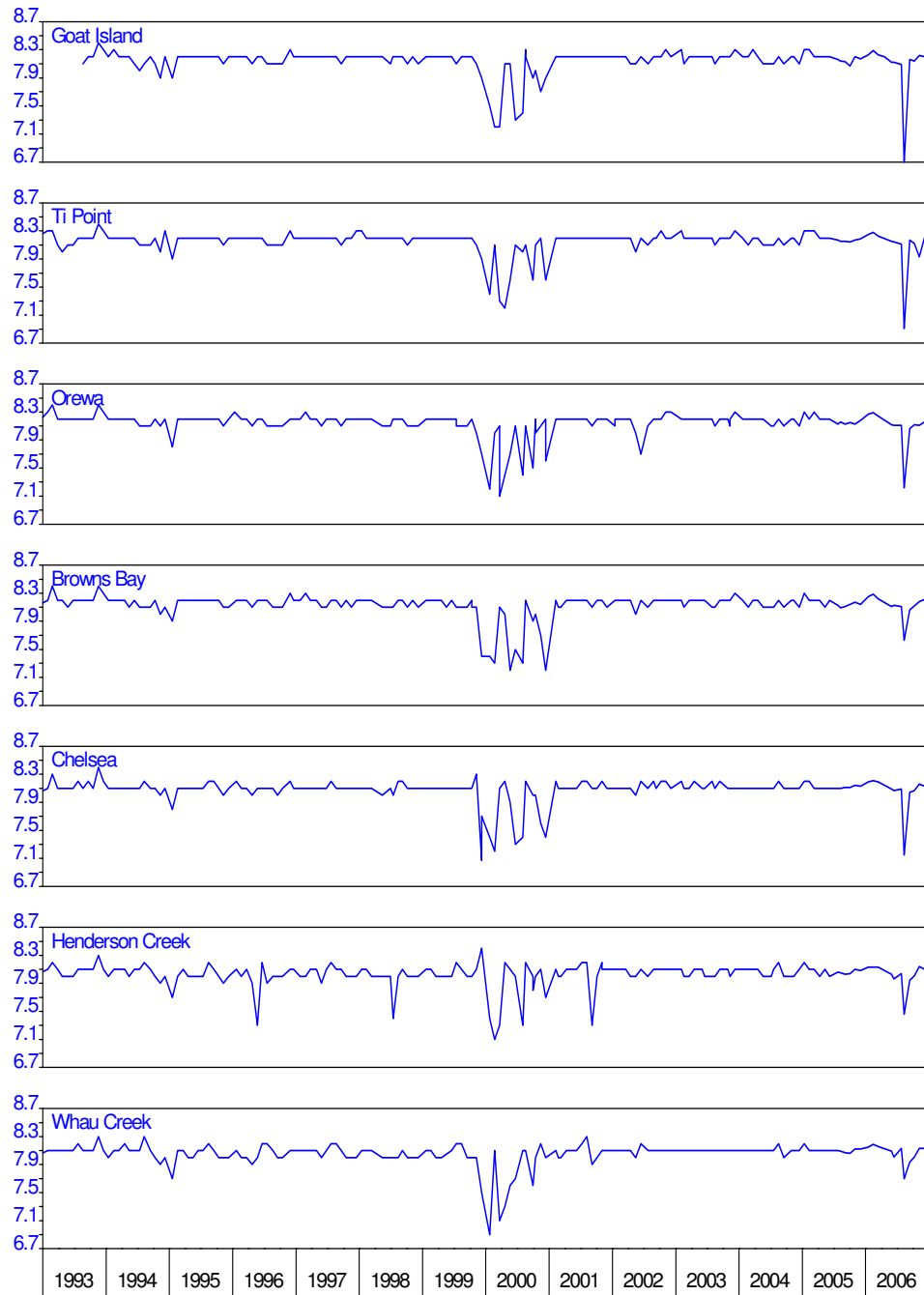
Figure 35: East Coast - pH
