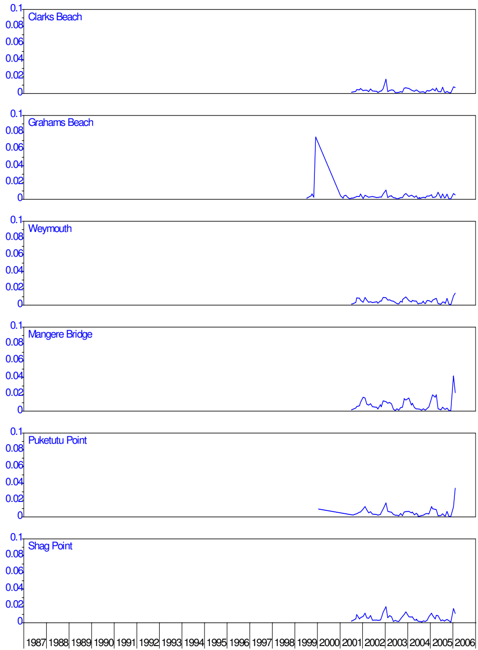
Figure 57: Manukau harbour – chlorophyll a (ppm)
