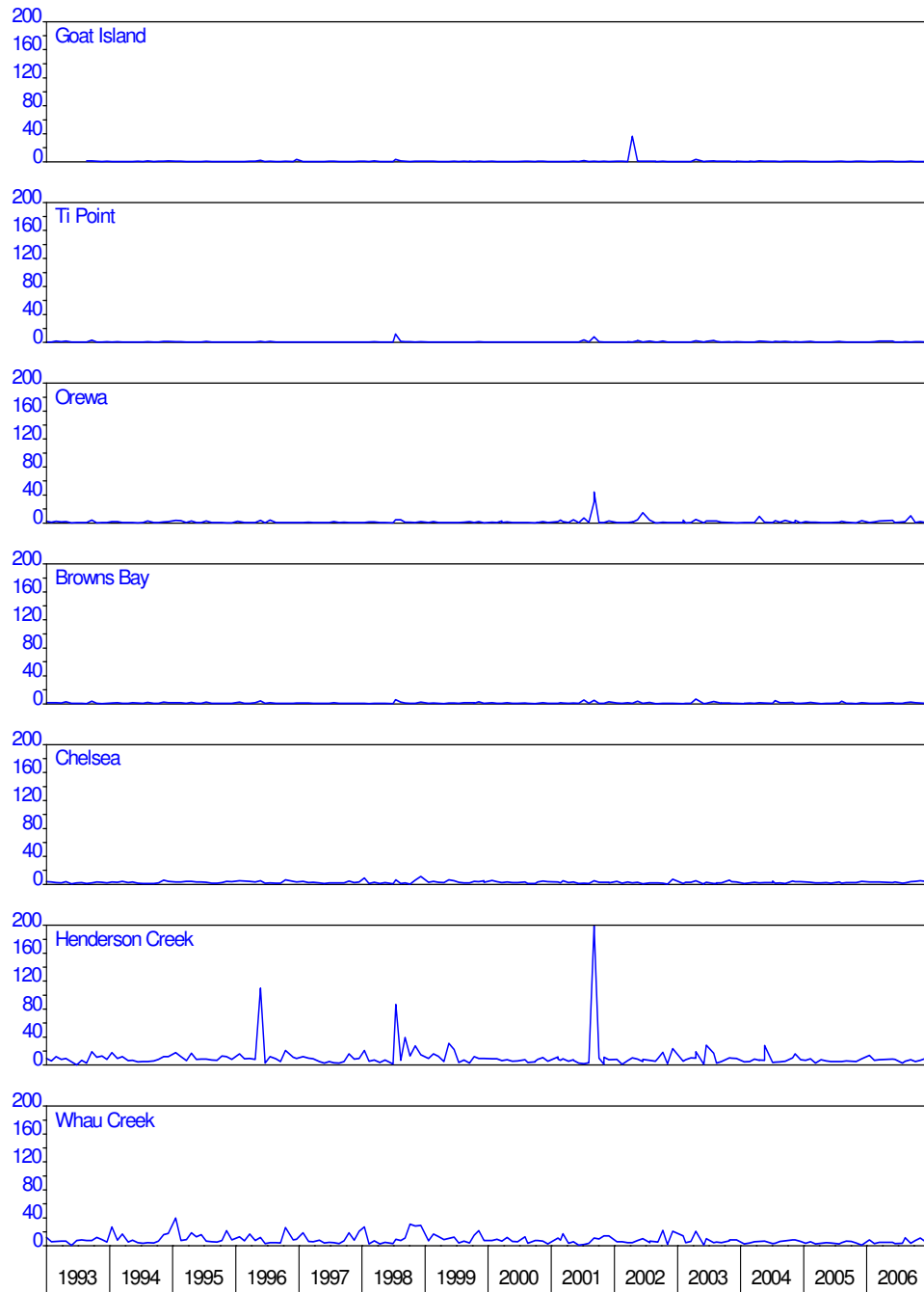
Figure 32: East Coast – turbidity (NTU)
