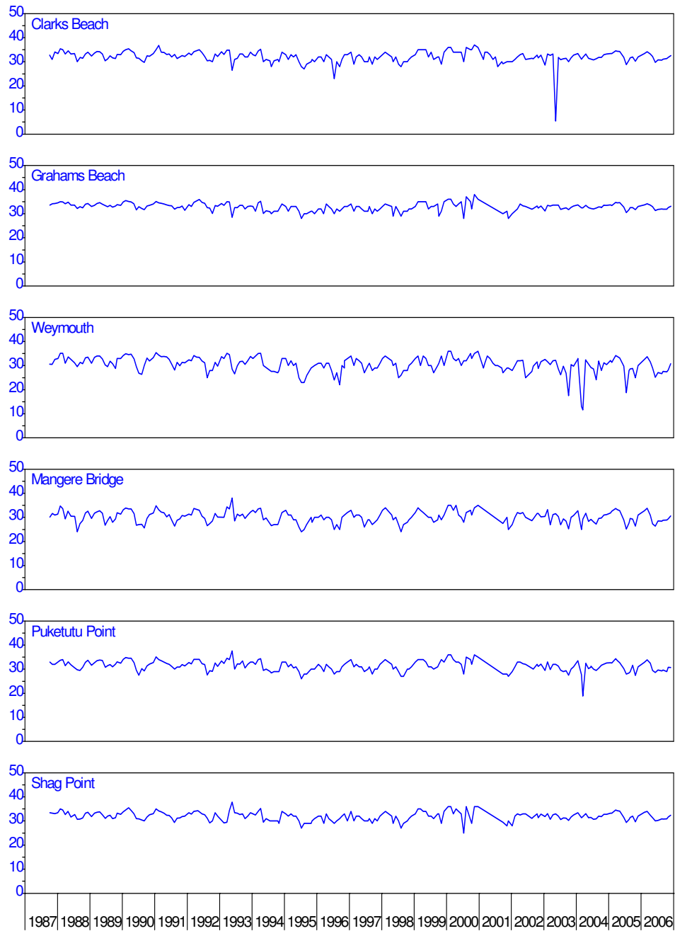
Figure 44: Manukau harbour – salinity (ppt)
