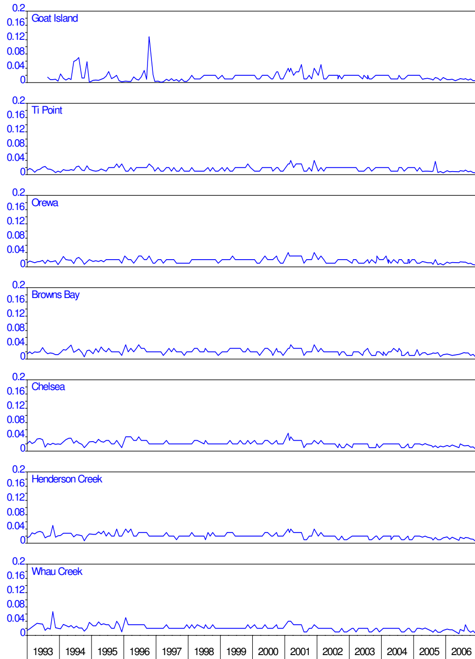
Figure 42: East Coast – dissolved reactive phosphorus (gP.m -3 )
