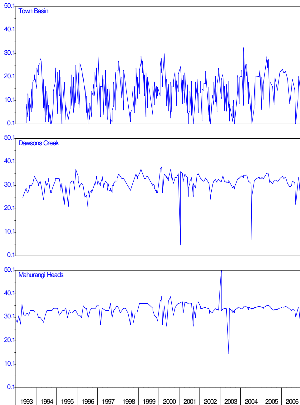
Figure 3: Mahurangi harbour – salinity (ppt)
