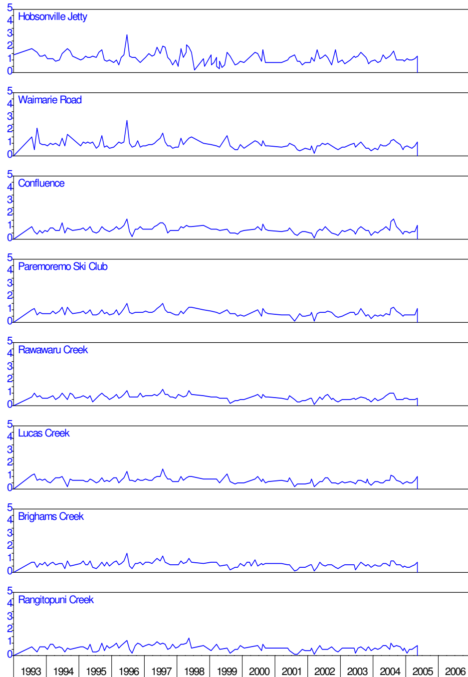
Figure 19: Upper Waitemata harbour – transparency (Secchi (m))
