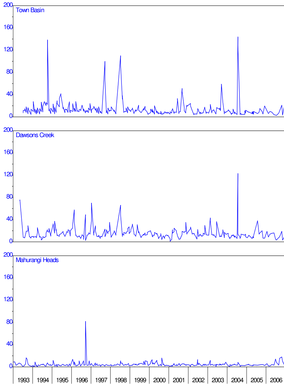
Figure 8: Mahurangi harbour – suspended solids (ppm)
